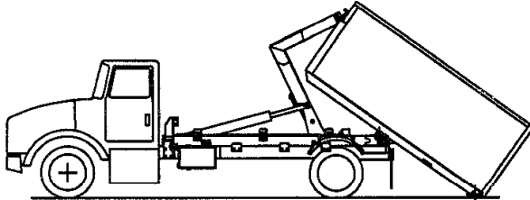
Max. Loading Angle 35 Deg.
