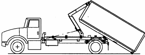
Max. Loading Angle 31 Deg.
