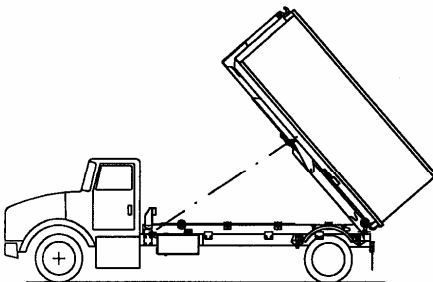
Max. Dumping Angle 49 Deg.
