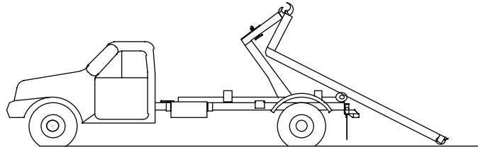
MAX. LOAD ANGLE 28 DEG
