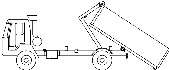
MAX. LOAD ANGLE 33 DEG
