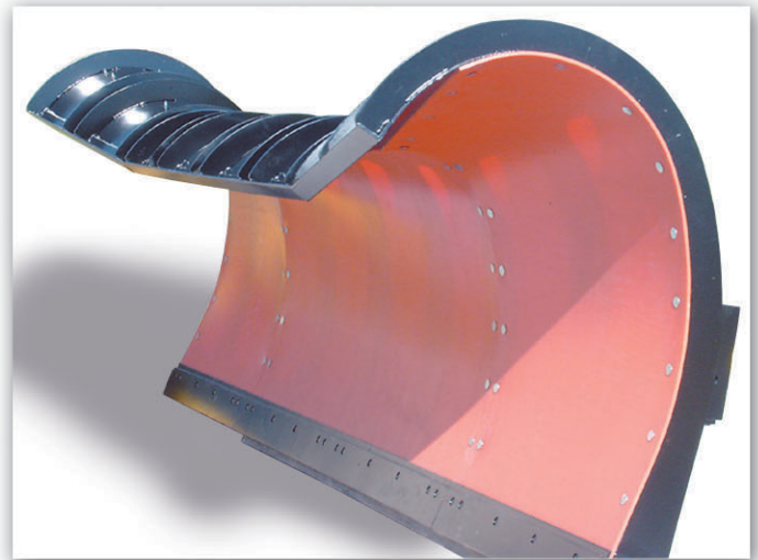
Integral Snow Deflector Prevents Snow Blowback
