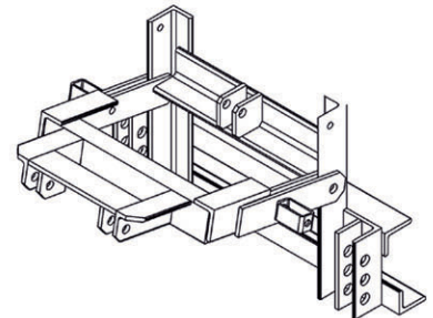
UH-LP-T - Universal Hitch Low Profile w/ Tilt ▲
