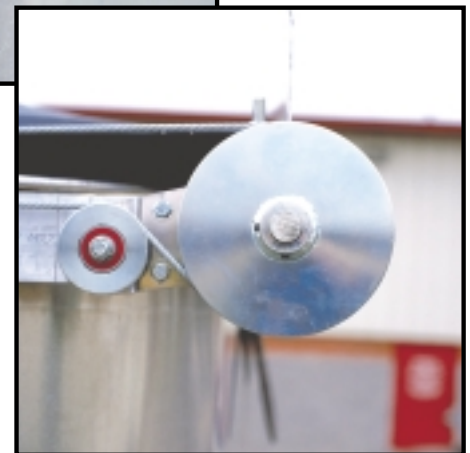
Second idler reduces cable slippage
