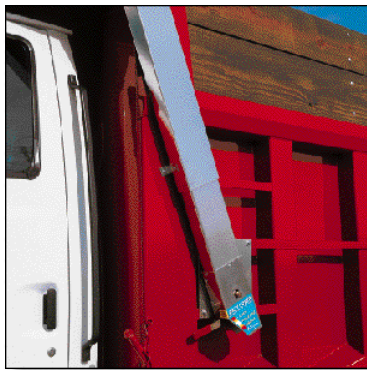
Ground Level: Model 400/450/475 Gives you the convenience of one-handed cranking from the ground.
