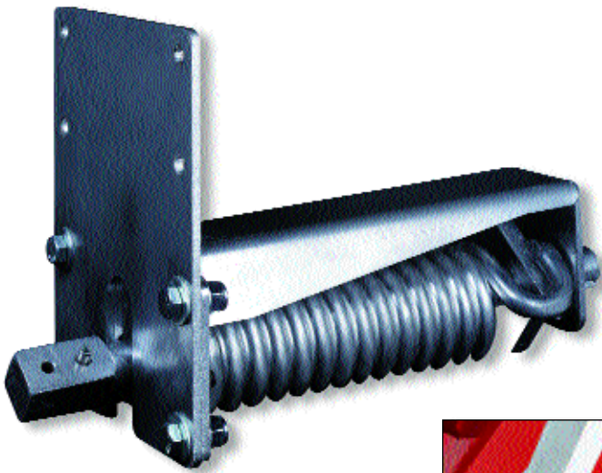
Undermount/Underbody Spring Assembly
